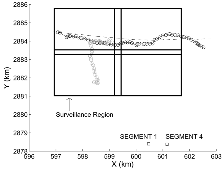
Fig. 12. Tracker target state point estimates. Two targets were automatically detected and tracked. A known truthed target was in the region (dashed). Notice that these track estimates are much more physically plausible than the track-fusion tracks.
